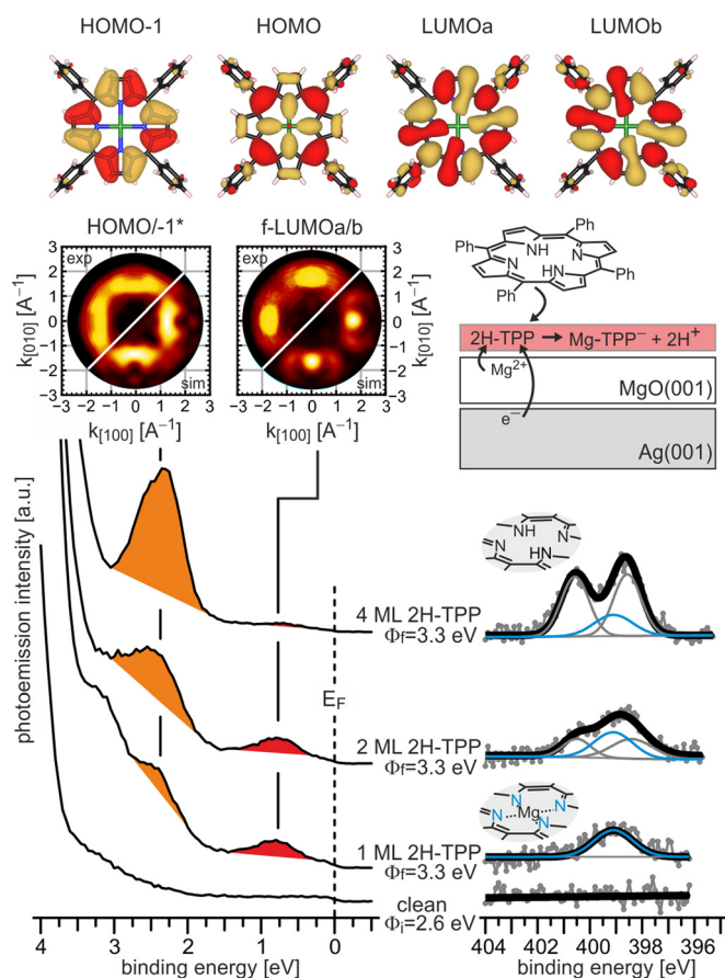
Figure 3. Top: real-space representation of the HOMO-1, HOMO, and the degenerate LUMOa and LUMOb of gas-phase Mg-TPP. ARUPS (bottom, left) and XPS (bottom, right) spectra of clean 2 ML MgO(001)/Ag(001) and increasing doses of 2H-TPP (1, 2, and 4 ML) at room temperature. Here, \Phi_i is the work function of clean MgO(001)/Ag(001) and \Phi_f is the work function after adsorption of 2H-TPP. Middle, left: comparison of experimental and simulated momentum maps of 1ML 2H-TPP on MgO(001)/Ag(001). The experimental maps were taken at the peak maxima of the PE peaks at 0.75 eV, showing the pattern of the superposition of the molecular LUMOa/b, and at 2.3 eV, showing the pattern of the superposition of the HOMO and HOMO-1. Middle, right: schematic model of charging and metalation upon adsorption of 2H-TPP on MgO(001)/Ag(001).
