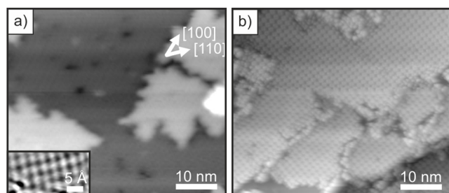
Figure 1. STM images of a) 2 ML MgO(001)/Ag(001) ( U_{\text{bias}} = 3.0 V, i_t = 29 pA), b) 1 ML 2H-TPP adsorbed on 2 ML MgO(001)/Ag(001) at room temperature and annealed at 473 K ( U_{\text{bias}} = 2.0 V, i_t = 28 pA). Inset in (a): atomically resolved image of MgO(001).
