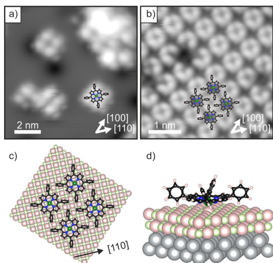
Figure 2. STM images of a) a low-coverage 2H-TPP film adsorbed at 80 K on 2 ML MgO(001)/Ag(001) ( U_{\text{bias}} = 1.2 V, i_t = 25 pA) and b) its ordered monolayer ( U_{\text{bias}} = 3.2 V, i_t = 55 pA). c) Tentative structural model of the monolayer phase derived from STM and LEED (top view). d) DFT-derived adsorption model of Mg-TPP on 2 ML MgO(001)/Ag(001) (3D view). In this model calculation charge transfer occurs from the substrate into the molecule.
