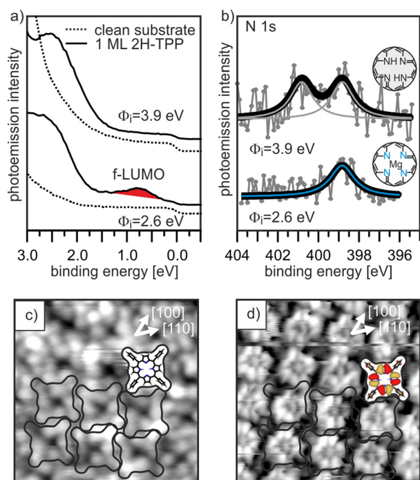
Figure 4. a,b) ARUPS (a) and N 1s XPS (b) for 2H-TTP adsorbed on 2 ML MgO(001)/Ag(001) films with different initial work function, \Phi_i . c,d) STM of 2H-TTP on high work function MgO(001)/Ag(001) at U_{\text{bias}} = +2.9 V (c) and U_{\text{bias}} = -2.6 V (d).
